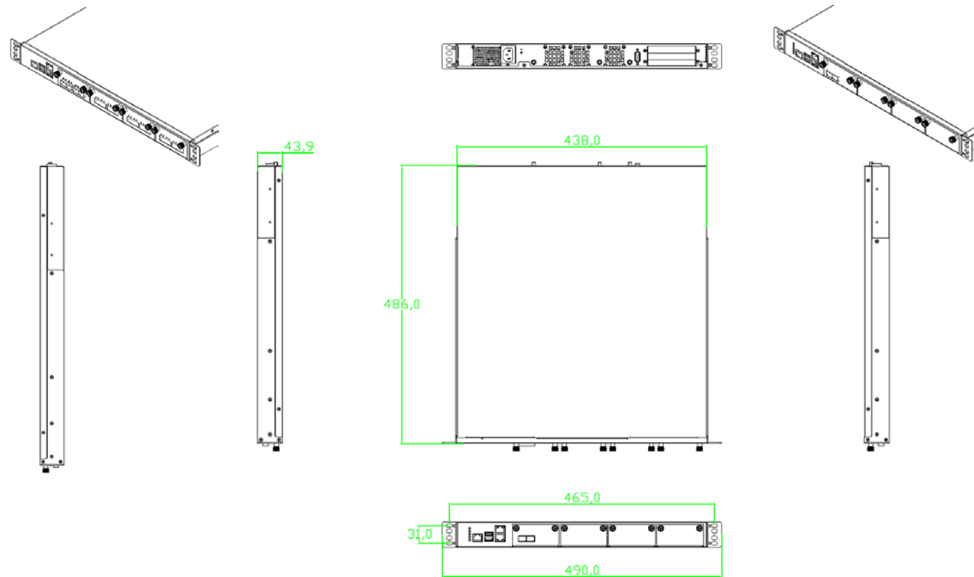
b. ATL-C236N4-SP
