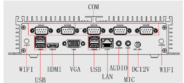
External I / O view of the rear panel
