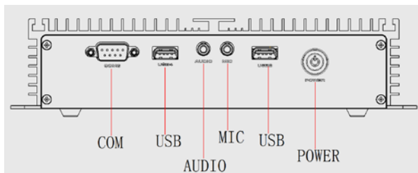
Front panel external I / O view
