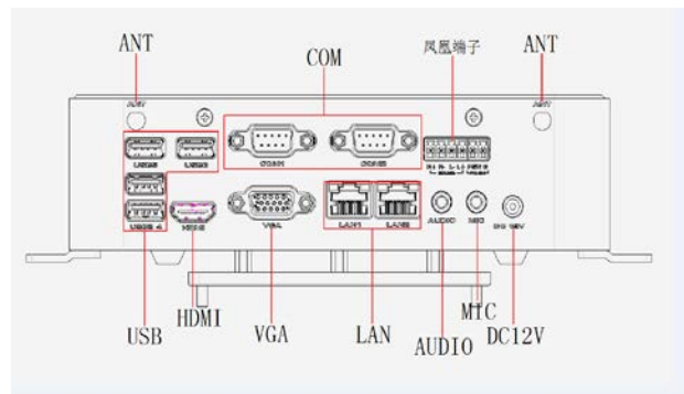
External I / O view of the rear panel
